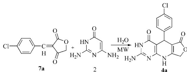
Scheme 4. The reaction between 7a and 2 in water under microwave irradiation conditions.
