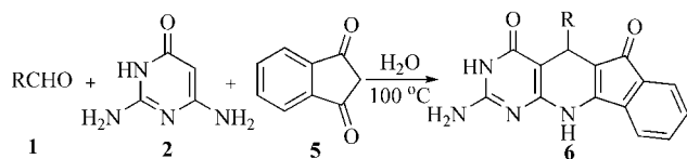
Scheme 2. Synthesis of 6 in water.
