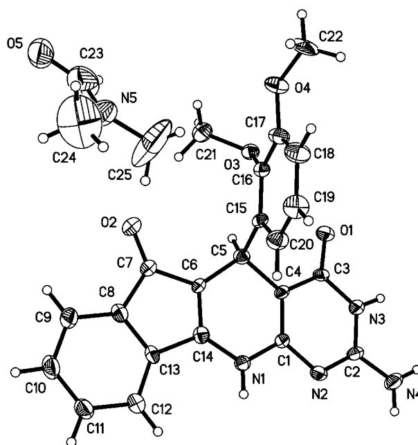
Figure 1. ORTEP diagram showing 6k .
