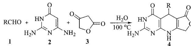
Scheme 1. Synthesis of 4 in water.
